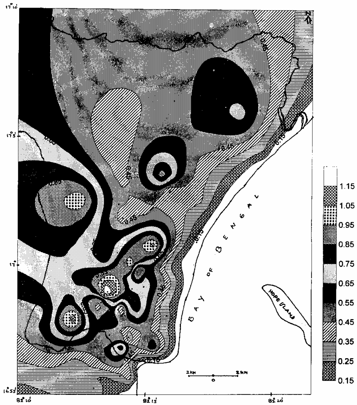
Fig.23. Spatial distribution of Sulphate/Chloride ratio in the study area (Nov. 99)
