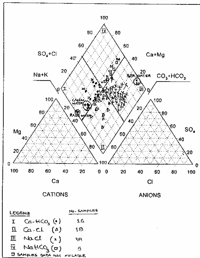
Fig. 13(a). Geochemical classification of different sources of samples (1 to 86) during Nov. 1999, Pipers (1953)
