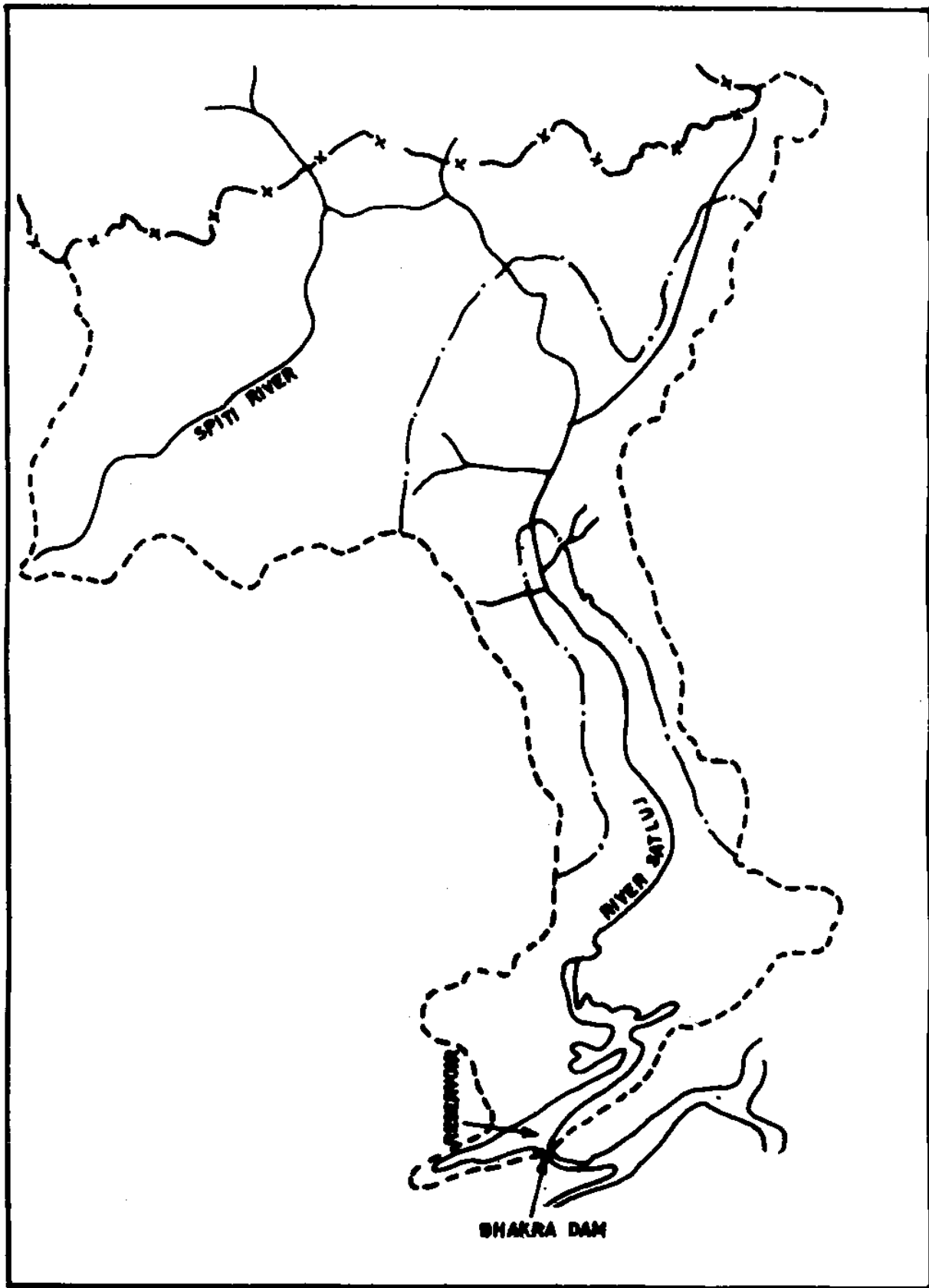
Fig. 3: Location of Spiti sub basin in the Satluj Basin
