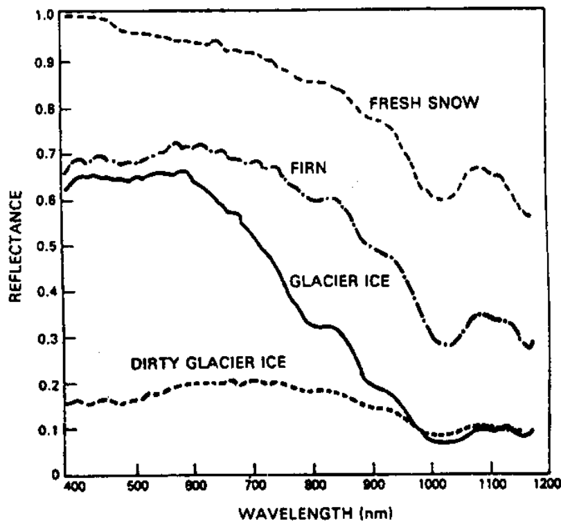
Fig. - 1 Reflectance Curves for Snow, Firn, Glacier and Dirty Ice
