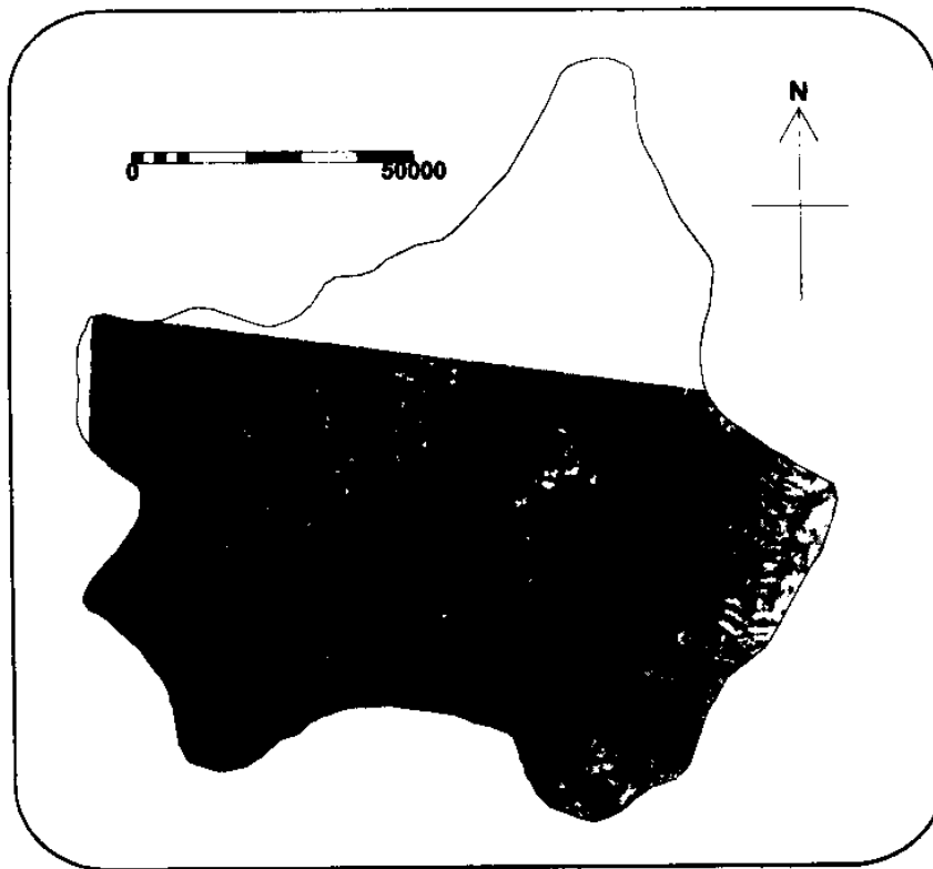
Fig. - 7 Georeferenced Band 4 image of IRS-1C LISS-III
