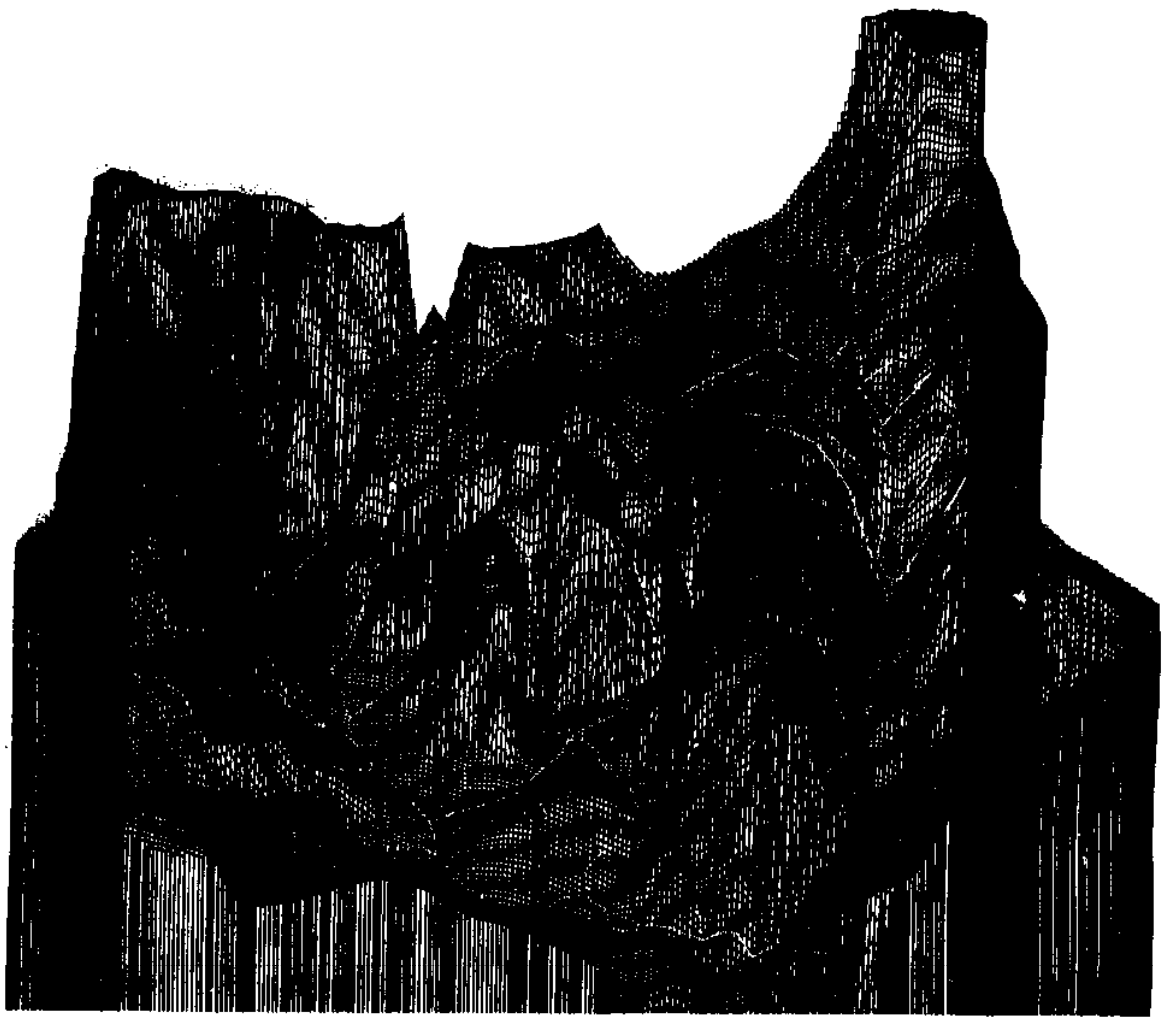
Fig. - 6 3-Dimensional View of the Spiti Basin
