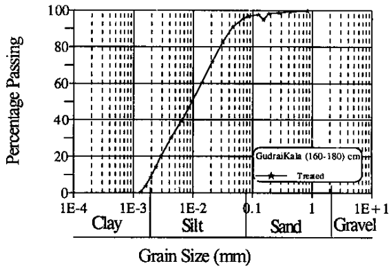
Fig. 8 Grain Size Distribution at Gudraikala
