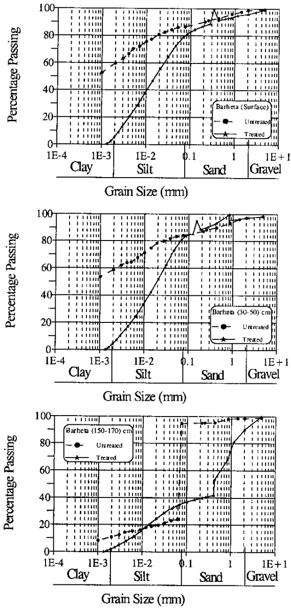
Fig. 9 Grain Size Distribution at Barheta
