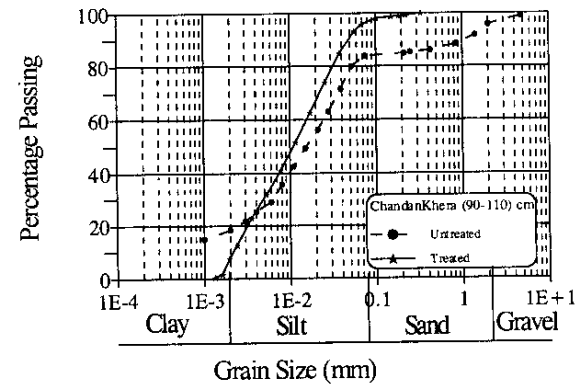
Fig. 15 Grain Size Distribution at Chandan Khera
