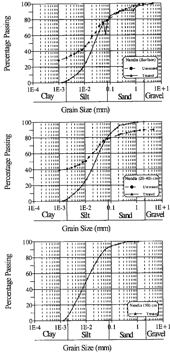
Fig. 14 Grain Size Distribution at Nandia
