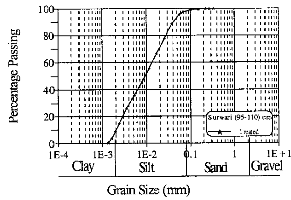
Fig. 10 Grain Size Distribution at Surwari
