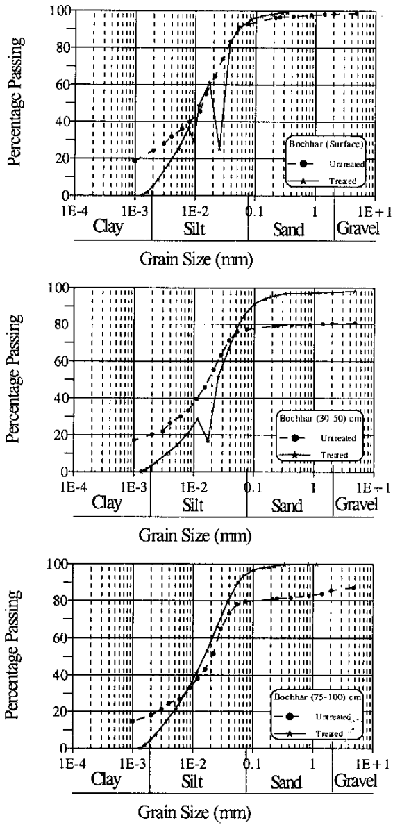
Fig. 11 Grain Size Distribution at Bochhar
