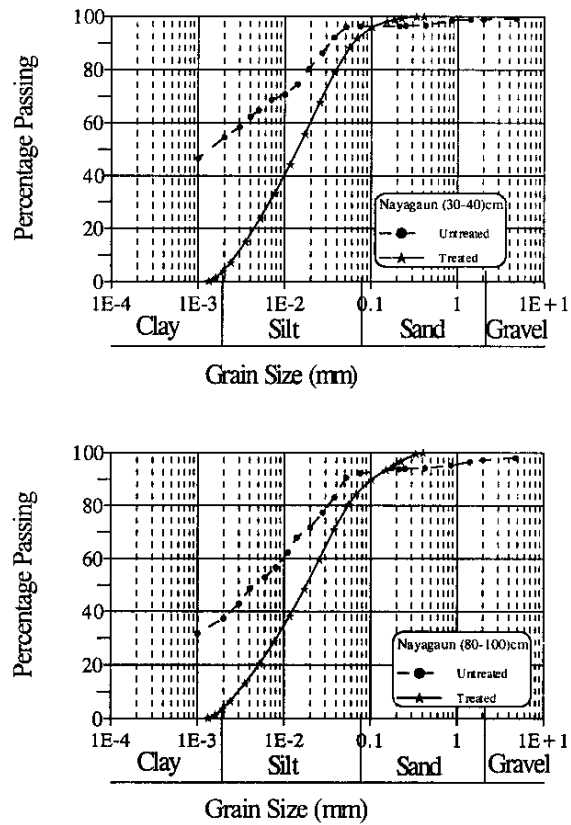
Fig. 5 Grain Size Distribution at Nayagaun
