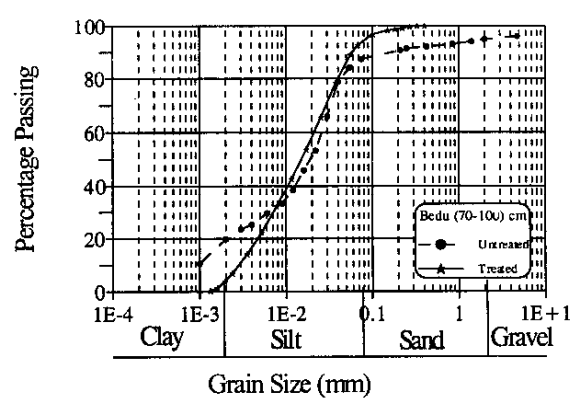
Fig. 7 Grain Size Distribution at Bedu
