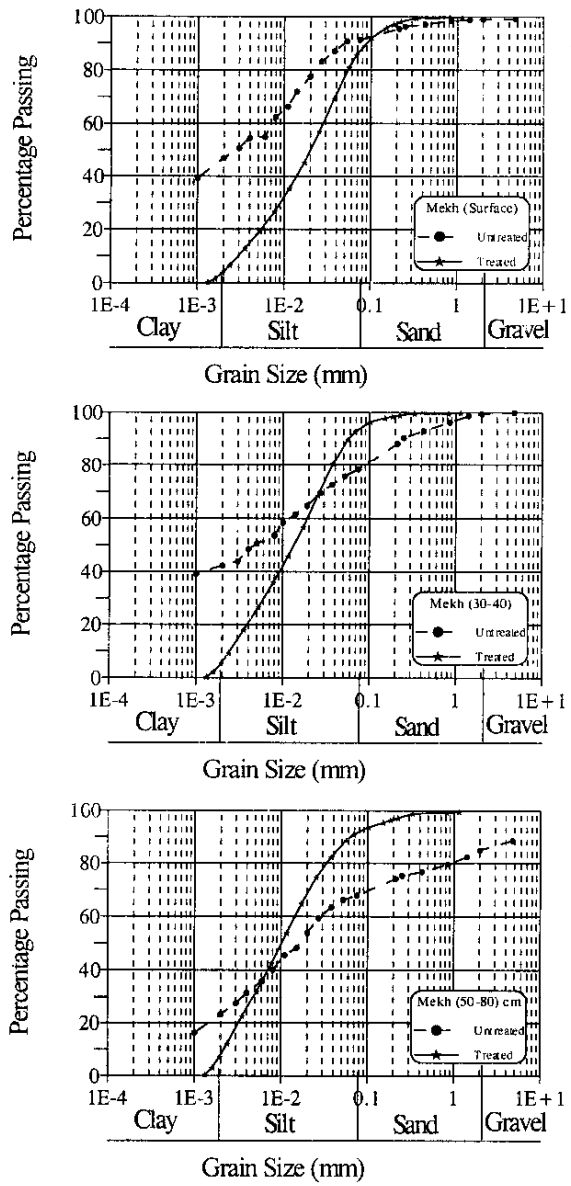
Fig. 12 Grain Size Distribution at Mekh
