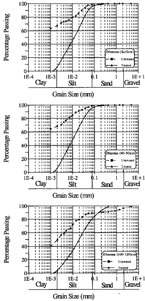
Fig. 6 Grain Size Distribution at Dhamma
