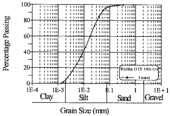
Fig. 16 Grain Size Distribution at Richha
