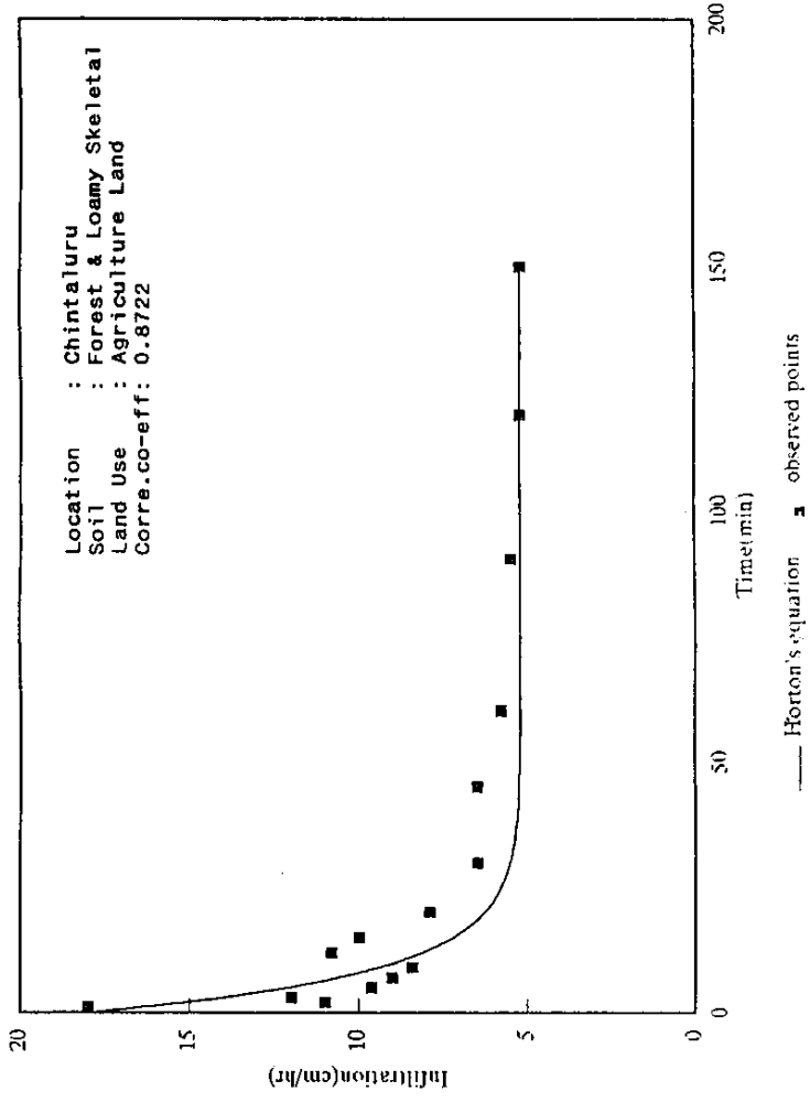
FIG. 28 HORTON'S INFILTRATION RATE CURVE
