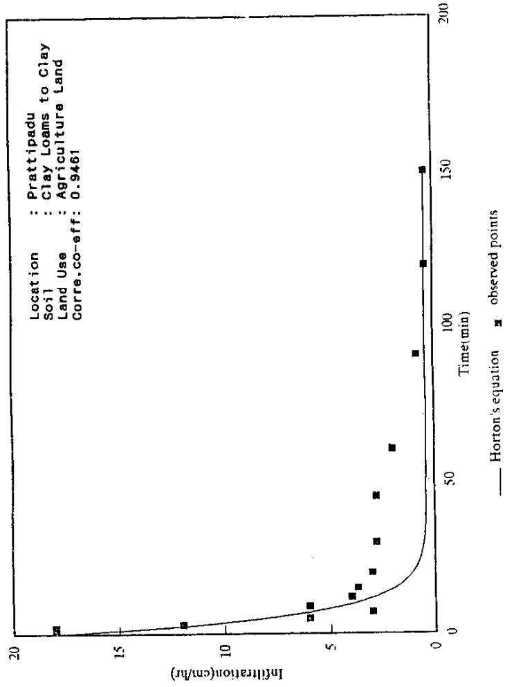
FIG. 12 HORTON'S INFILTRATION RATE CURVE
