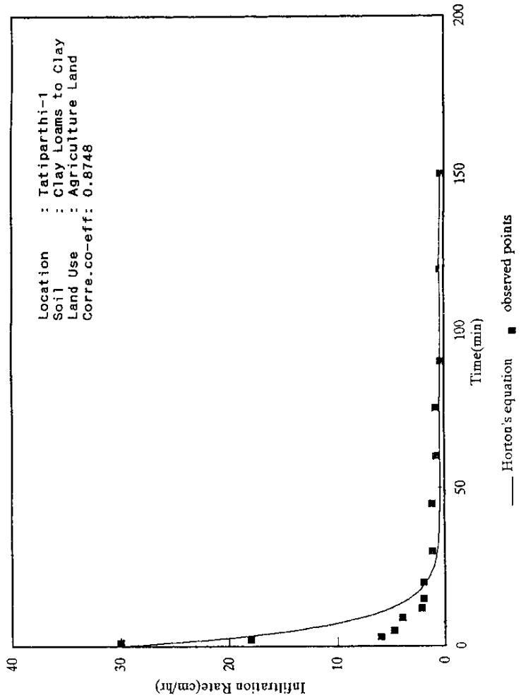
FIG. 8 HORTON'S INFILTRATION RATE CURVE
