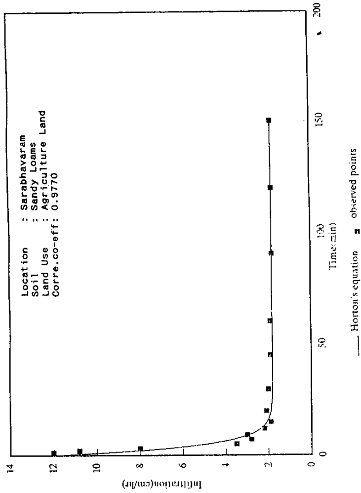
FIG. 24 HORTON'S INFILTRATION RATE CURVE
