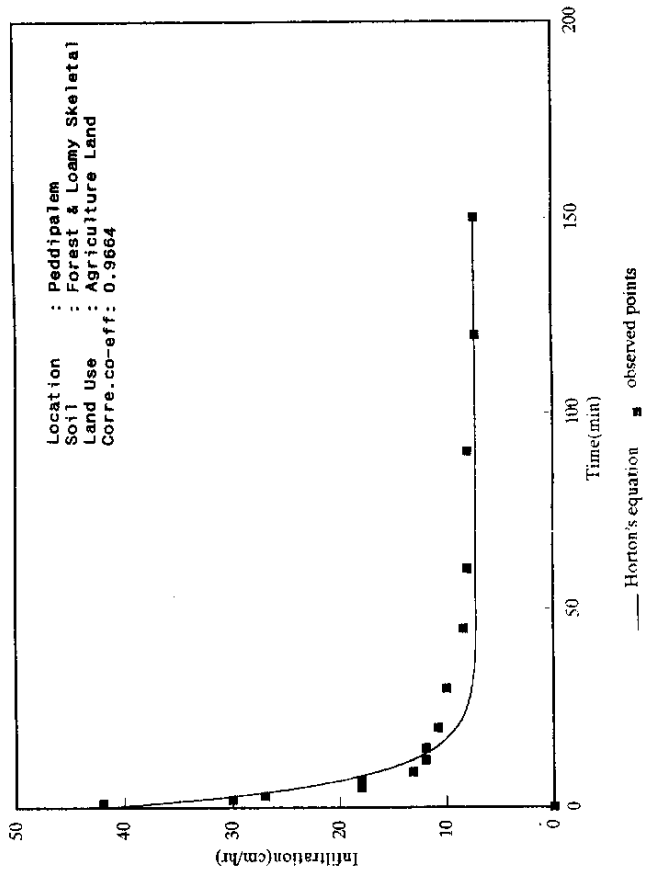
FIG. 29 HORTON'S INFILTRATION RATE CURVE
