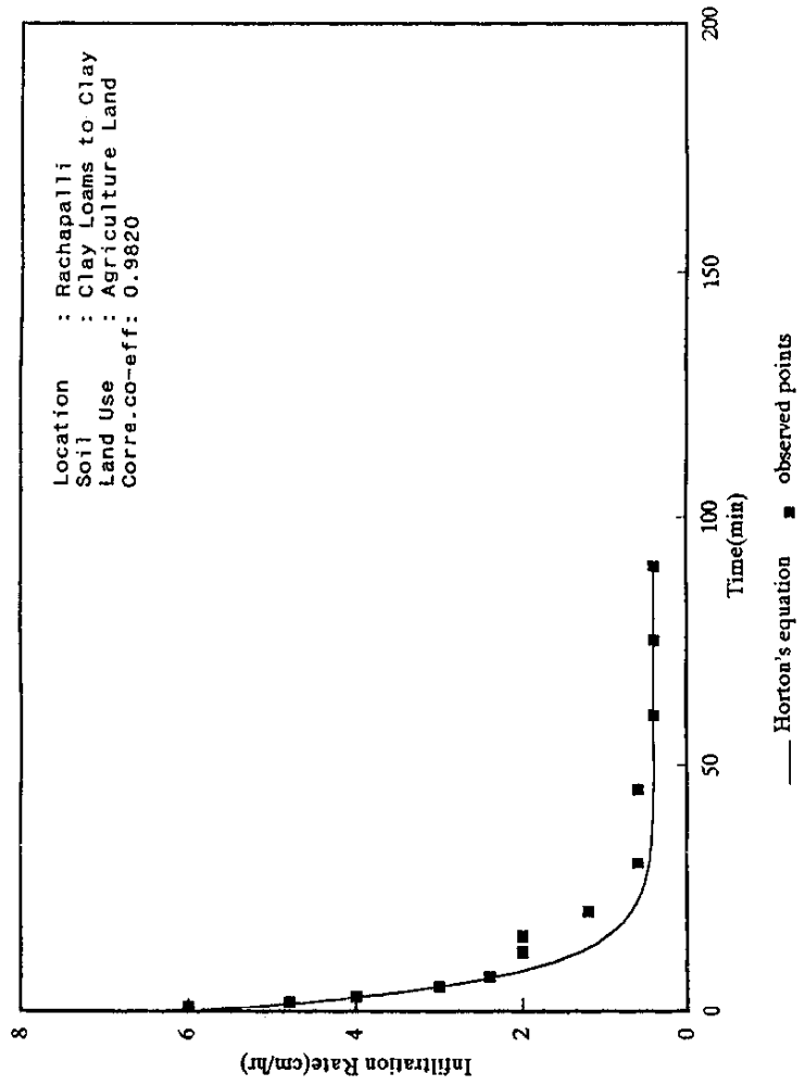
FIG. 7 HORTON'S INFILTRATION RATE CURVE
