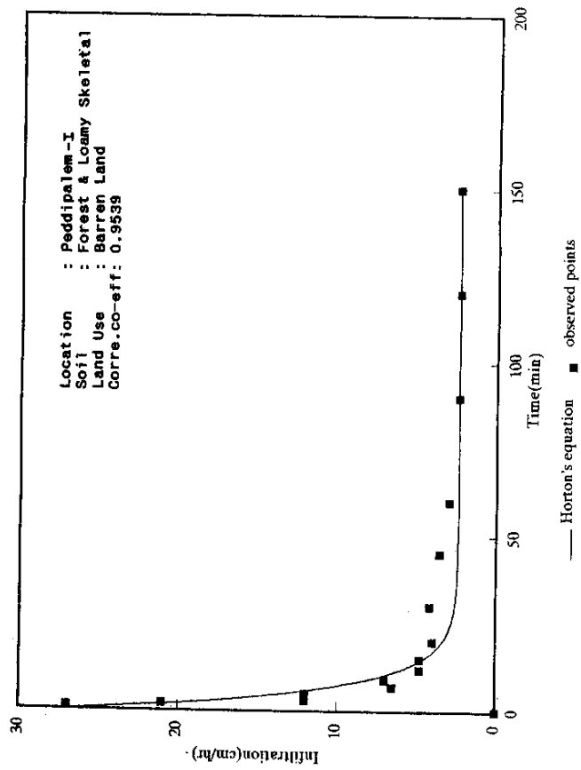
FIG. 30 HORTON'S INFILTRATION RATE CURVE
