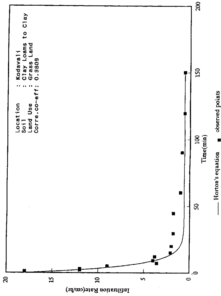
FIG. 15 HORTON'S INFILTRATION RATE CURVE
