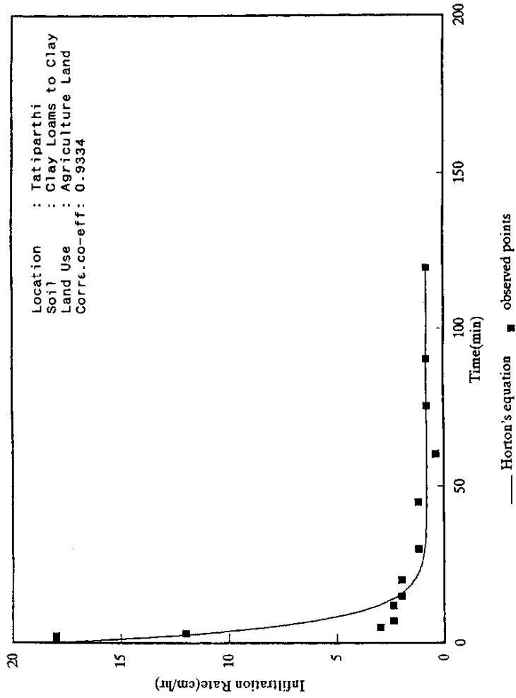
FIG. 9 HORTON'S INFILTRATION RATE CURVE
