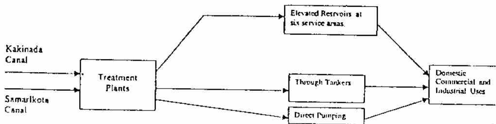
Fig. No. : 3 Schematic Flow Diagram of Kakinada Water Supply System
