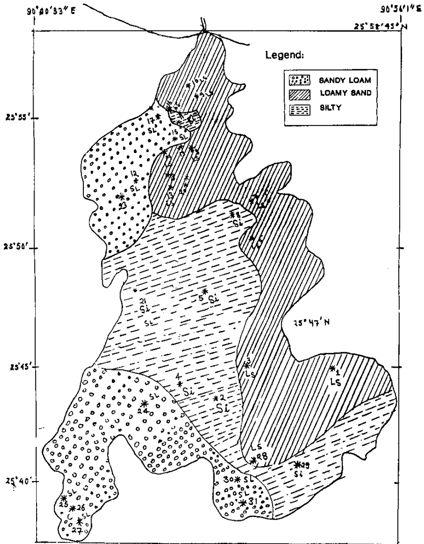
Fig.2 HYDROLOGIC SOIL CLASSIFICATION FOR DUDHNA BASIN BASED ON TEXTURE AND STRUCTURE
