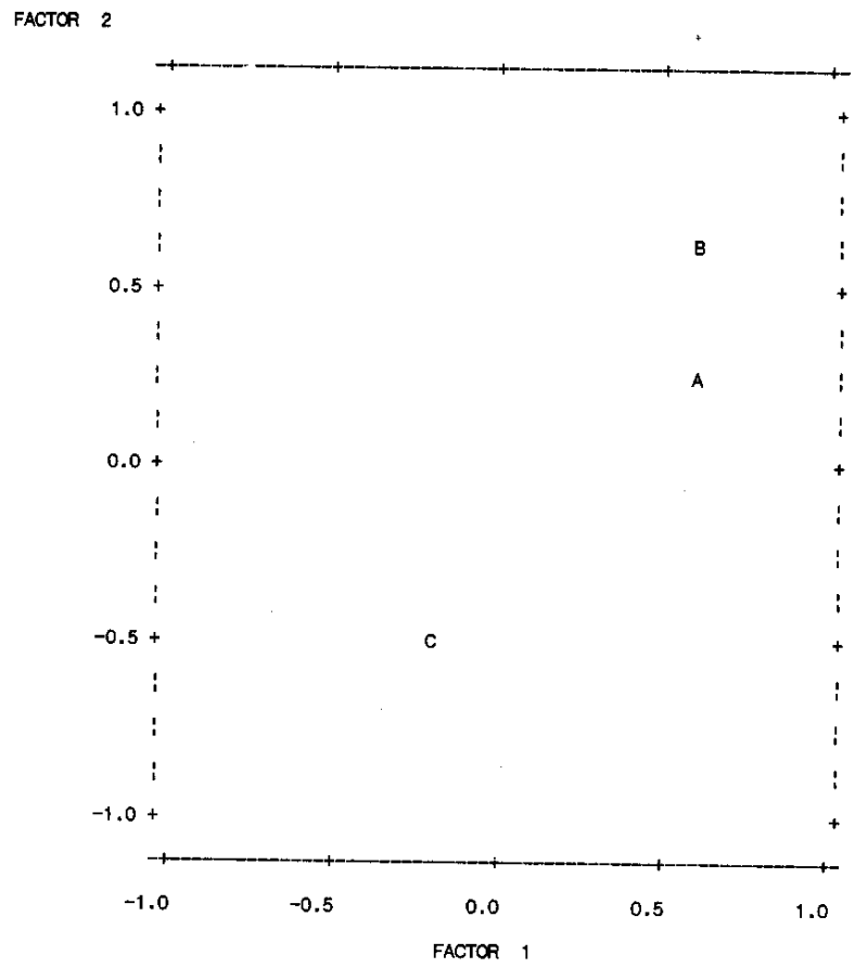
Fig.11 FACTOR LOADING PLOTS
