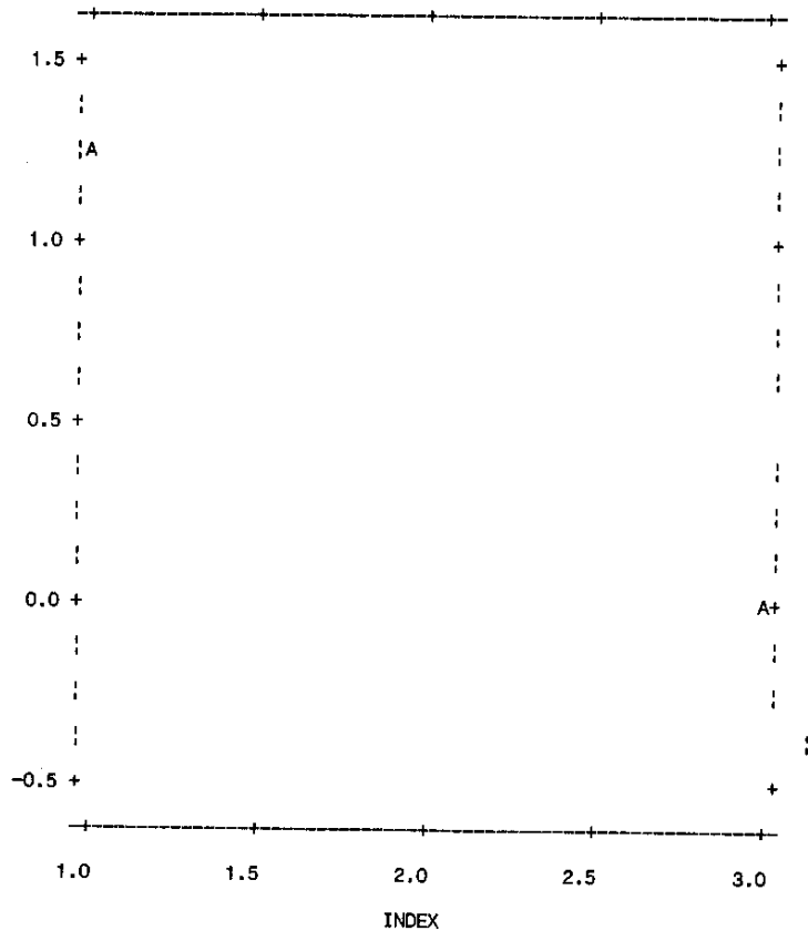
Fig.10 FACTOR SCREE PLOT
