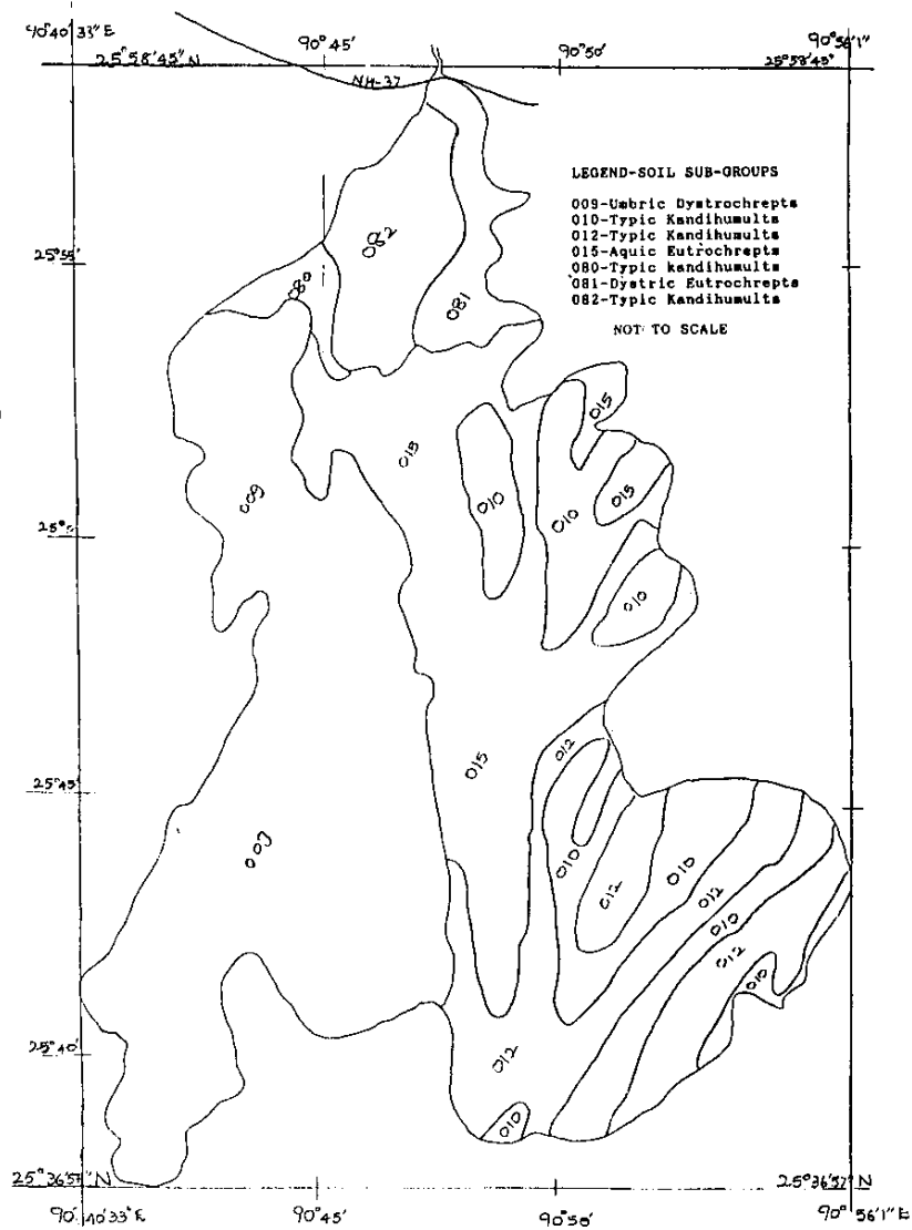
Fig.6 SOIL RESOURCES INVENTORY. Source : NBSS & LU
