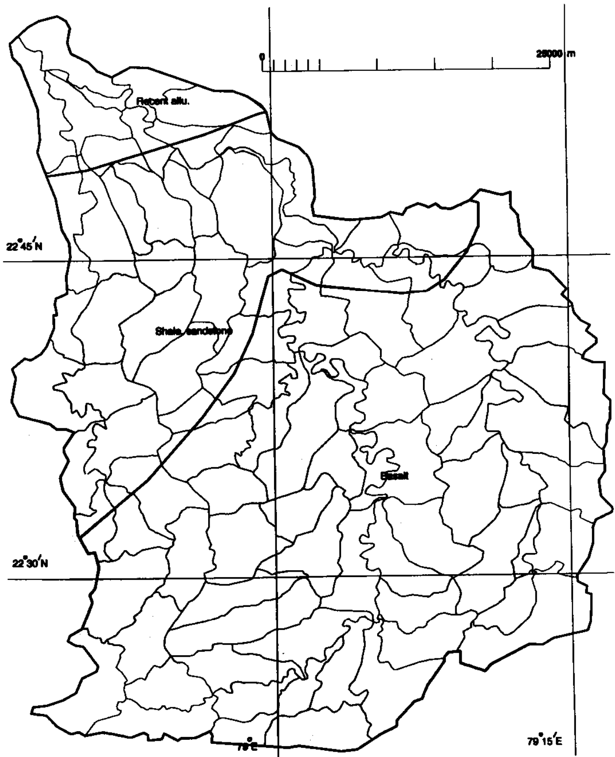
Fig. 5.5 Geology
