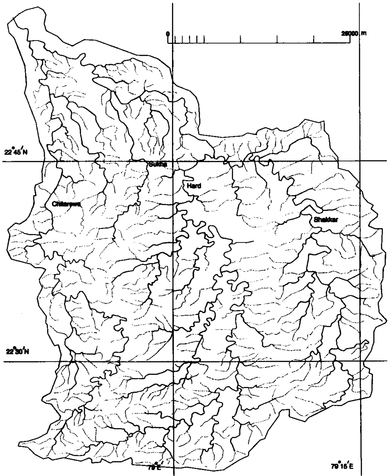
Fig. 3.1 Study area
