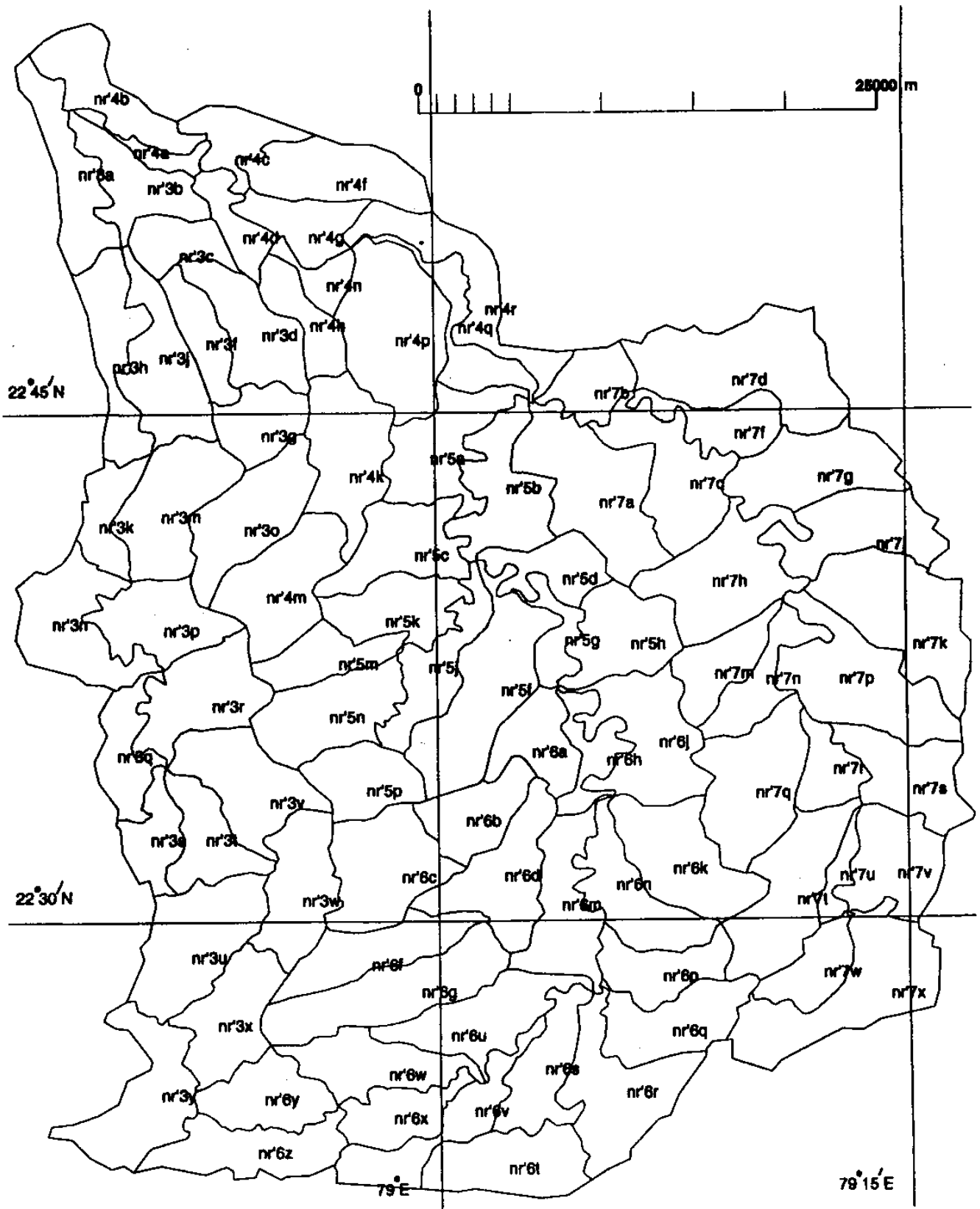
Fig. 5.1 Subwatersheds
