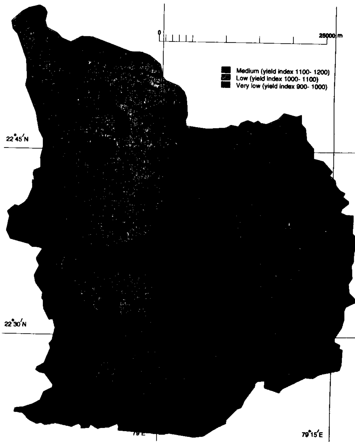
Fig. 5.6 Subwatersheds priority
